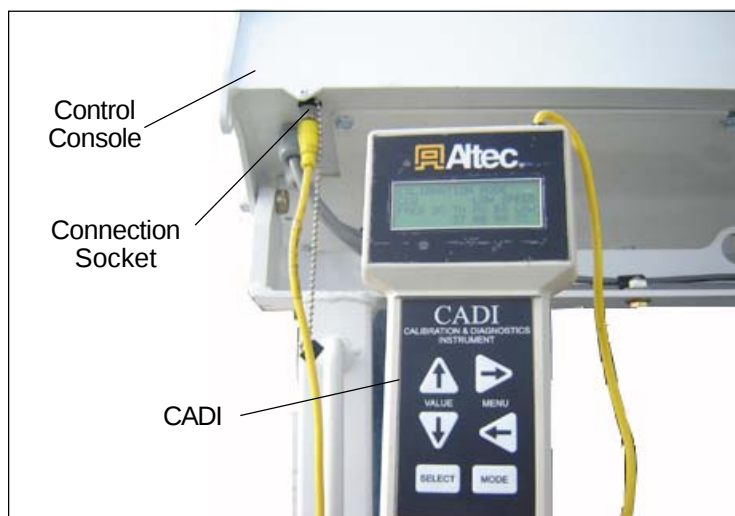
Figure 7 - CADI Attached to Connection Socket
