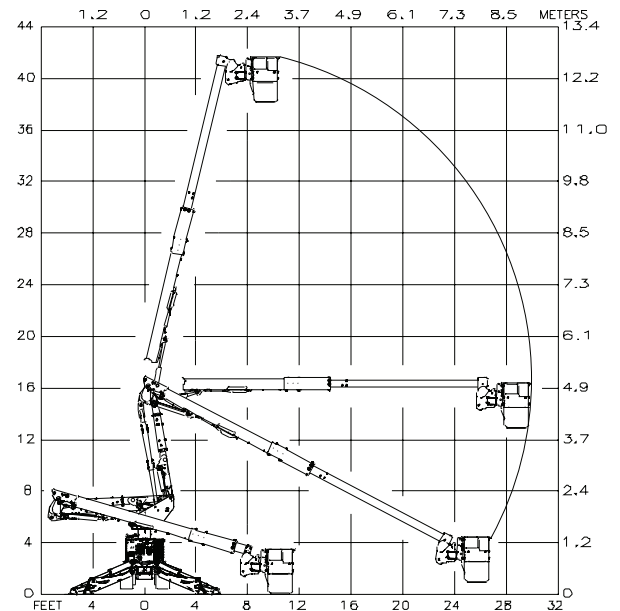
AT40-CW REACH DIAGRAM
